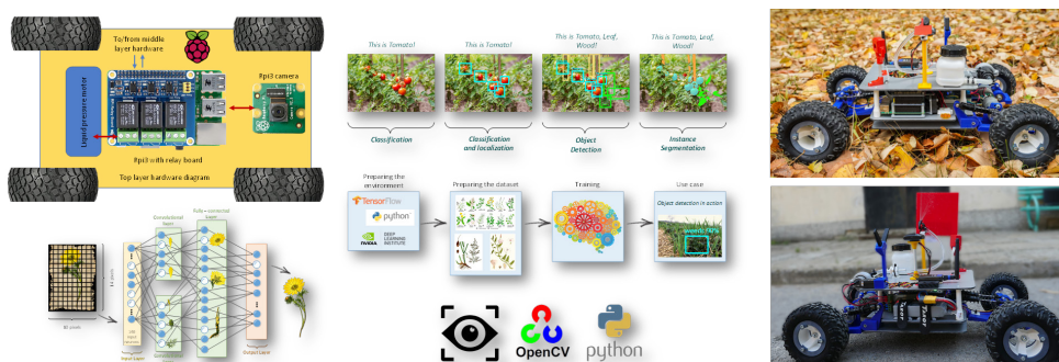
Figure 2. The AgRUBot robotic prototype – a small-scale solution for precision agriculture that utilizes a CV-based AI algorithm for weed detection and spraying
