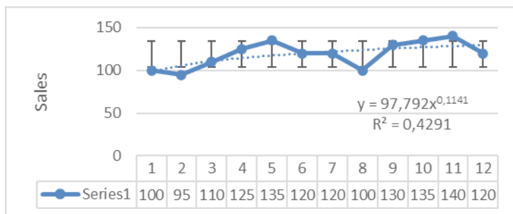
Figure 15. Power function
