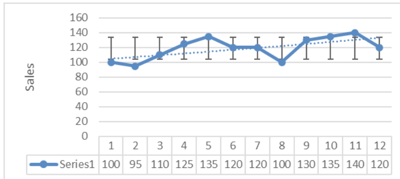
Figure 10. Exponential fuction
