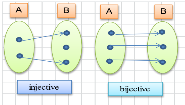
Figure 3. Injective, Bijective
