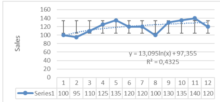
Figure 13. Logarithmic function
