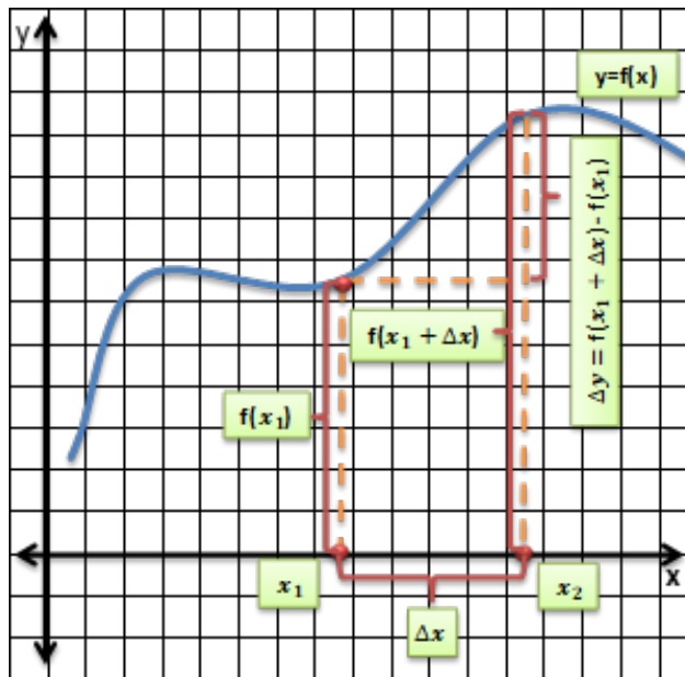
Figure 5. Monotonicity
