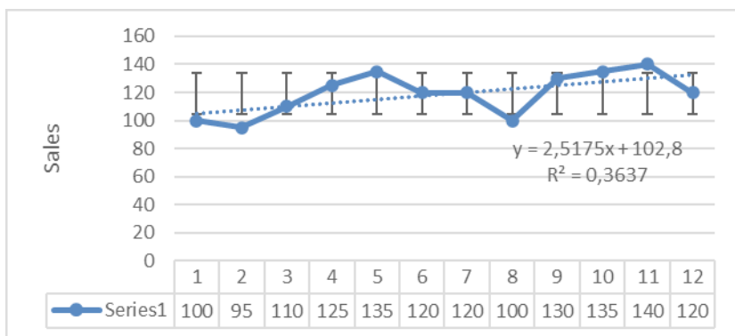
Figure 12. Linear function
