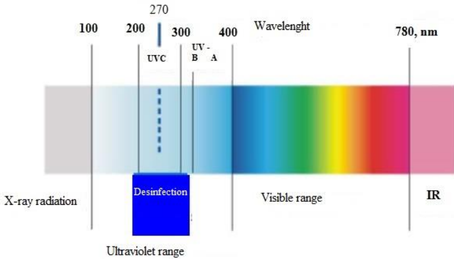
Figure 2. Electromagnetic waves
