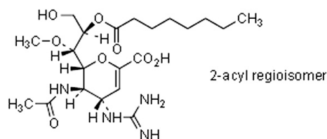
6. Laninamivir octanoate
