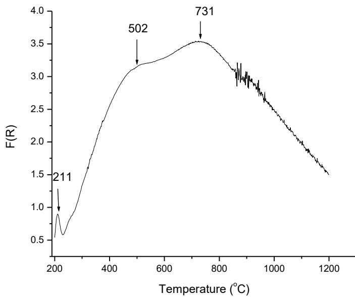
Fig. 7. Electronic spectrum for complex C2
