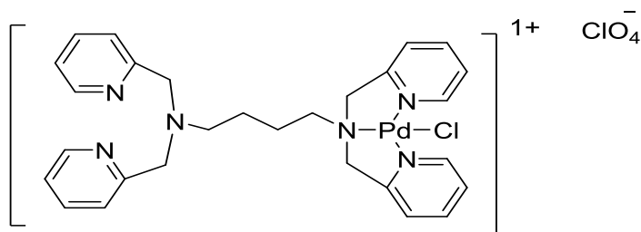
Pd[N,N,N,N-Tetrakis(2-pyridyl methyl)1,4-butanediimine]Cl(ClO 4 )
