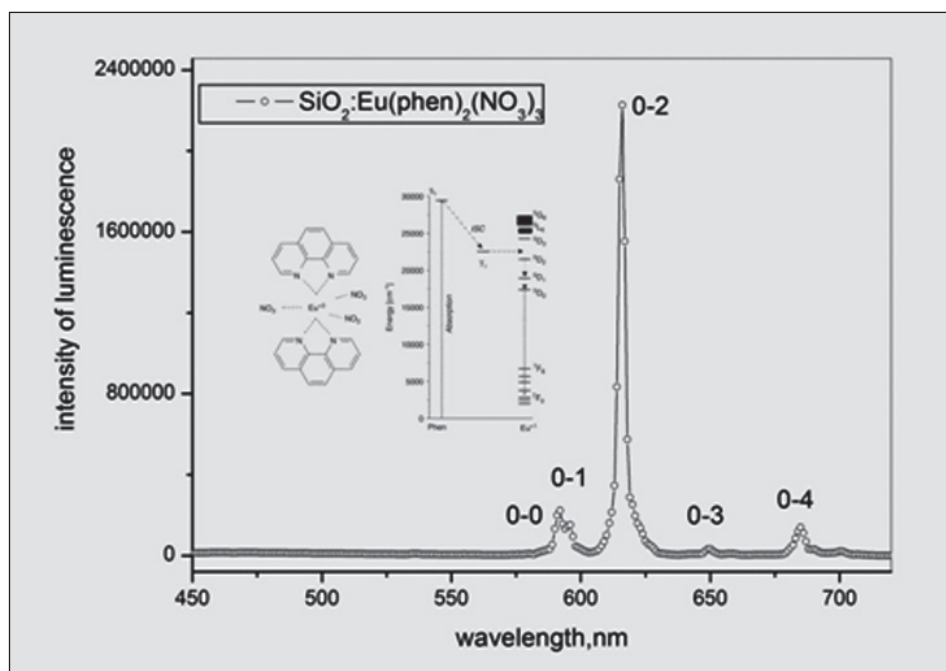
Fig. 4. A typical luminescence spectrum of \text{SiO}_2:[\text{Eu}(\text{phen})_2](\text{NO}_3)_3 powders at 352 nm excitation. The \text{Eu}^{3+} \ ^5\text{D}_0 \rightarrow ^7\text{F}_{0,1,2,3,4} transitions are denoted as 0-1,2,3,4. The optical properties of the complex are shown (Görrler-Walrand & Binnemans, 1998)
