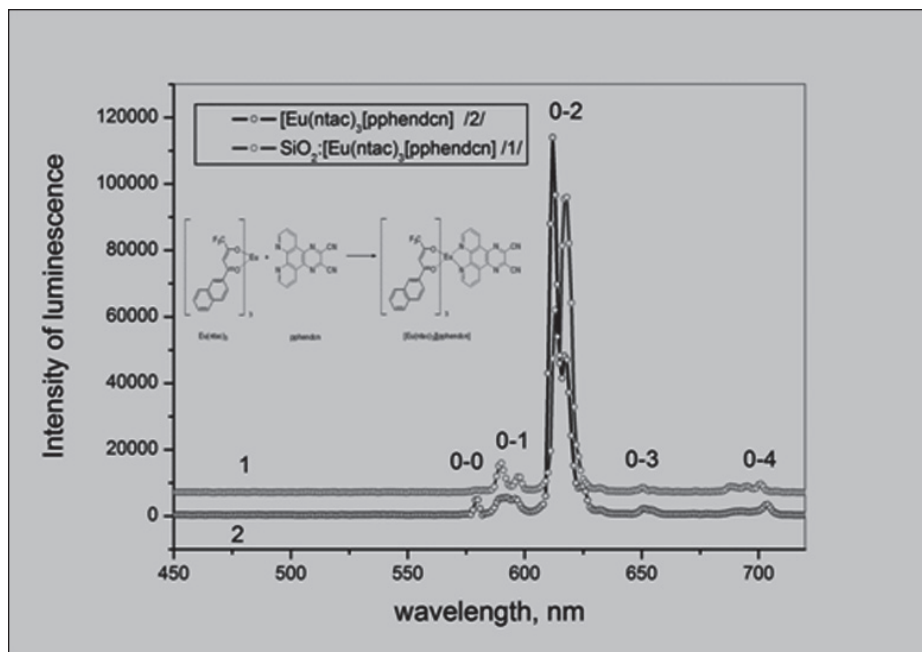
Fig. 6. Luminescence spectra of [\text{Eu}(\text{ntac})_3][\text{pphendcn}] and functionalized \text{SiO}_2:[\text{Eu}(\text{ntac})_3][\text{pphendcn}] at 400 nm excitation. The \text{Eu}^{3+} {}^5\text{D}_0 \rightarrow {}^7\text{F}_j transitions are denoted as 0-1, 0-2, 0-3 and 0-4
