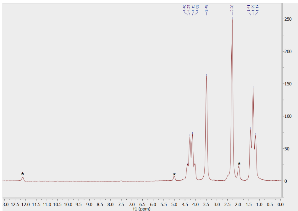
Figure 5. ^1\text{H} NMR spectrum of compound B collected in Chloroform-D. Peaks marked with an asterisk belong to the enol form
