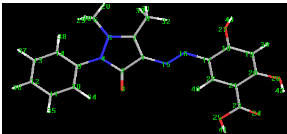
Figure 1. Optimised geometry of the ligand
