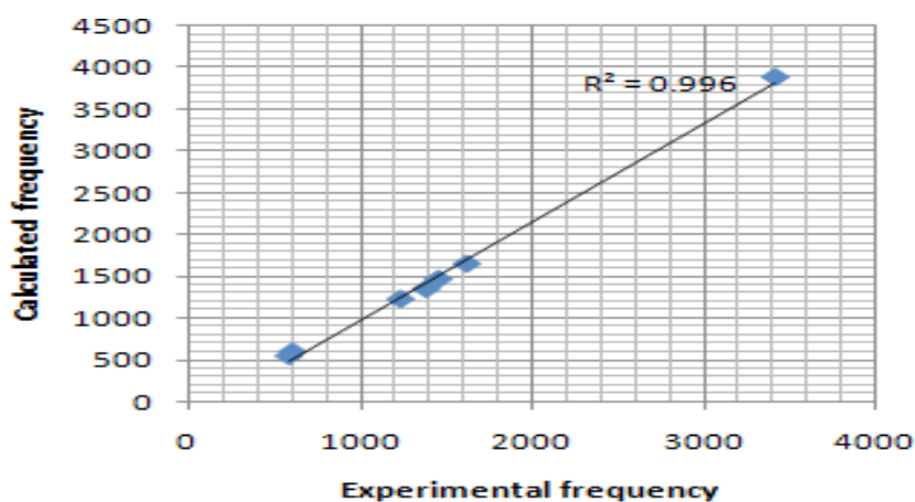
Figure 11. Correlation Graph between experimental and calculated frequency (PM3) of the Co(II) complex
