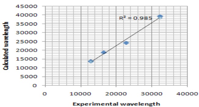
Figure 19. Correlation graph between calculated and experimental wavelength of Co(II) complex
