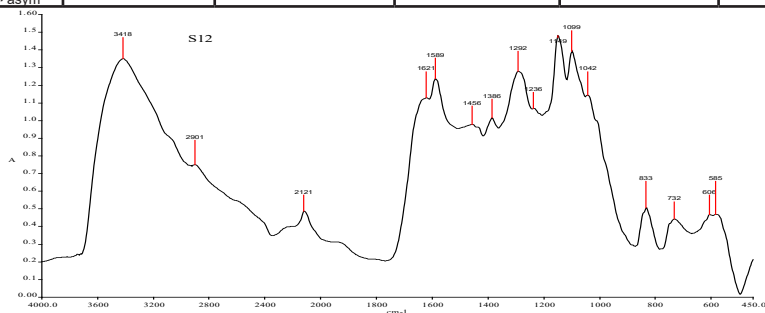
Figure 5. IR spectrum of the Co(II) complex
