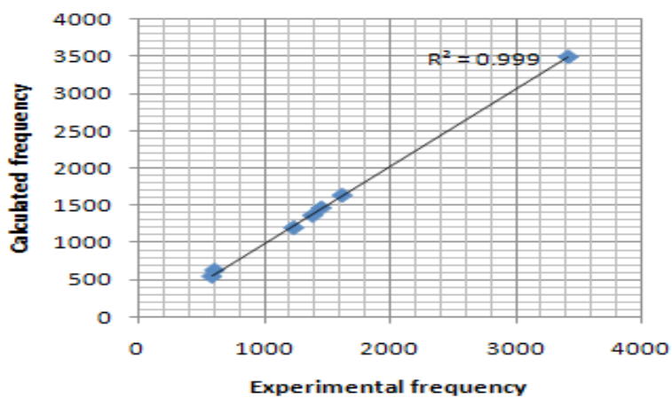
Figure 10. Correlation Graph between experimental and calculated frequency (AM1) of the Co(II) complex
