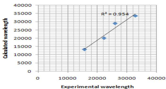
Figure 20. Correlation graph between calculated and experimental wavelength of Ni(II) complex
