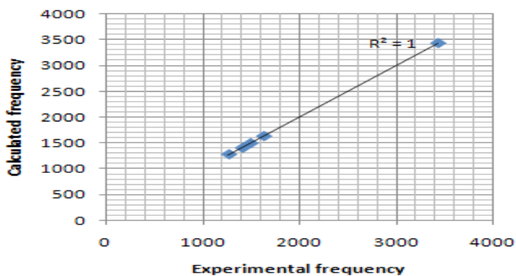
Figure 6. Correlation Graph between experimental and calculated frequency
