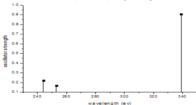
Figure 17. Calculated electronic spectrum of the ligand
