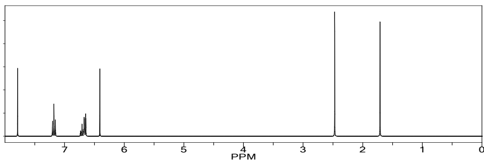
Figure 16. Calculated NMR spectra of the Zn(II) complex
