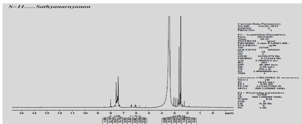
Figure 15. Experimental NMR spectra of the Zn(II) complex
