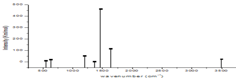
Figure 8. Calculated vibration frequency of the Co(II) complex by AM1 method
