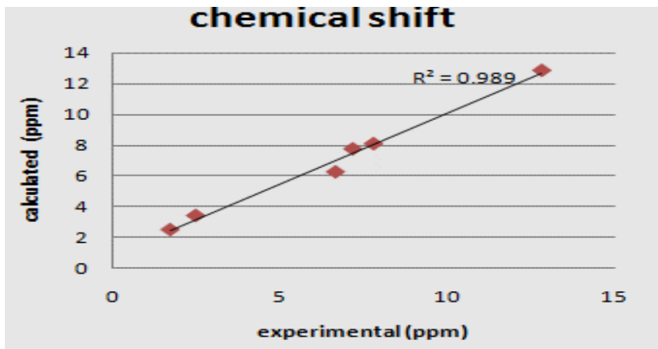
Figure 17. Correlation graph between calculated and experimental chemical shifts of the ligand
