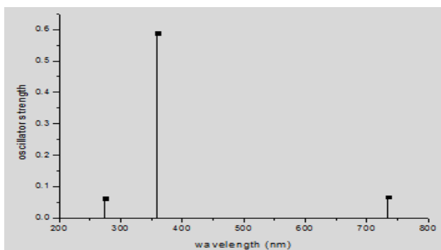
Figure 18. Calculated electronic spectrum of the Cu(II) complex
