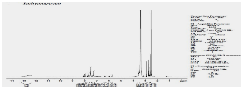
Figure 13. Experimental NMR spectra of the ligand
