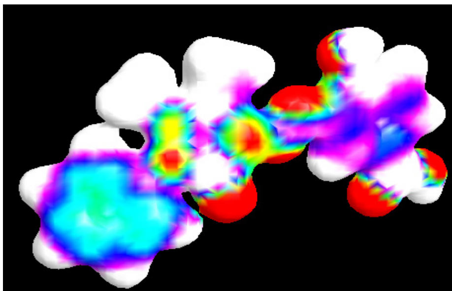
Figure 3. MEP of the ligand
