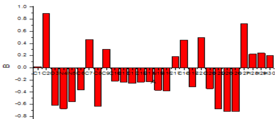
Figure 2. Histogram of Mulliken charge of the ligand
