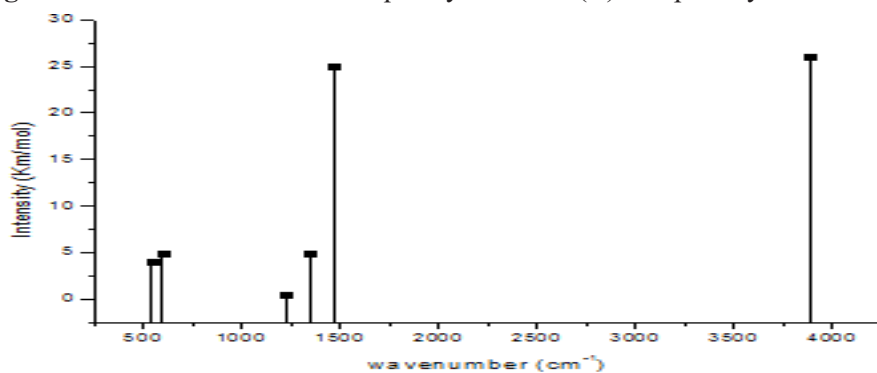
Figure 9. Calculated vibration frequency of the Co(II) complex by PM3 method
