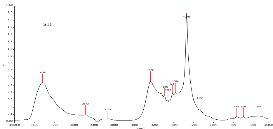
Figure 4. IR spectrum of the ligand
