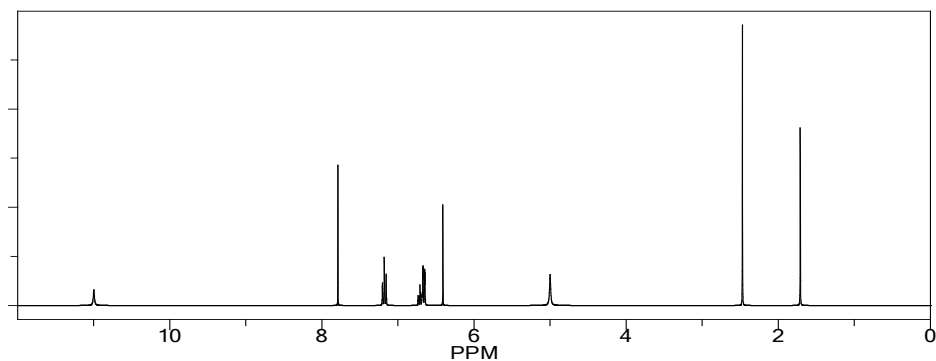
Figure 14. Calculated NMR spectra of the ligand
