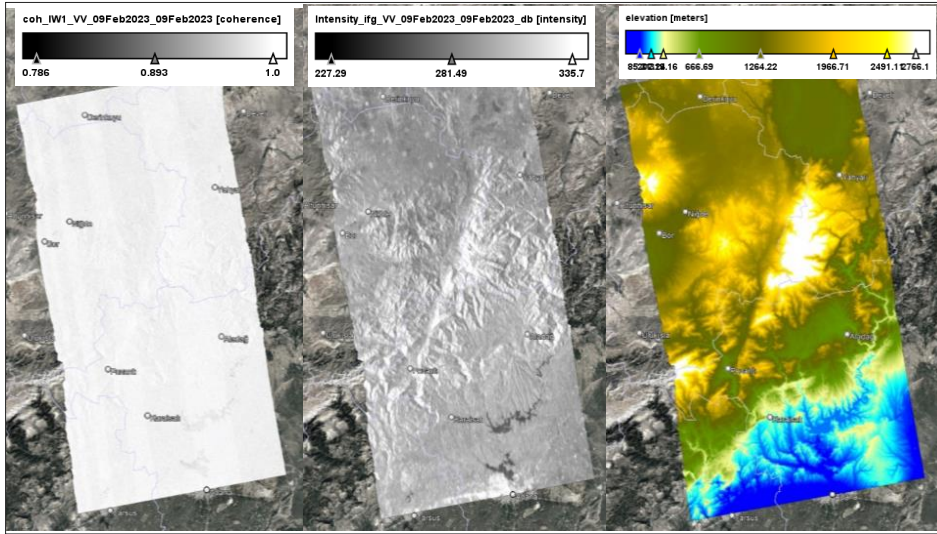
Figure 9. Coherence (left panel). Intensity (central panel). DEM (right panel) Orbit 14: 28.01.2023-9.02.2023
