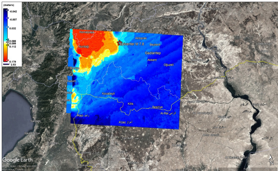
Figure 10. Deformation map using images from Orbit 21. The earthquake epicenter is denoted as red star
