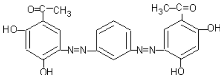
Fig. 2. Structure of ligand-L/H 4 -1,3-bis(2',4'-dihydroxy-5'-acetylphenylazo)benzene
