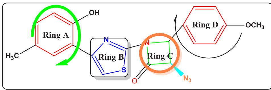
Figure 8. Structure-activity relationships substituted 3-azido-4-phenyl-1-(4-phenylthiazole-2-yl)azetidin-2-one ( 3a-s )
