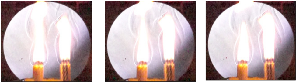
Figure 12. Different stages of flame puffing, N = 7, r = 3.6 cm
