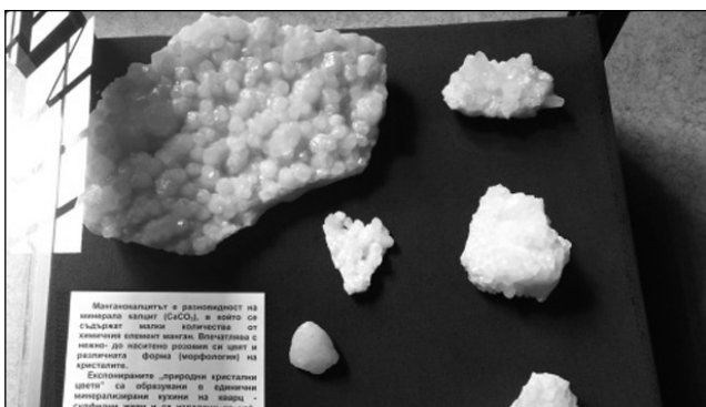
Figure 7. Manganocalcite, (\text{Ca,Mn})\text{CO}_3 is a variety of calcite rich in manganese, which gives the mineral a pink color
