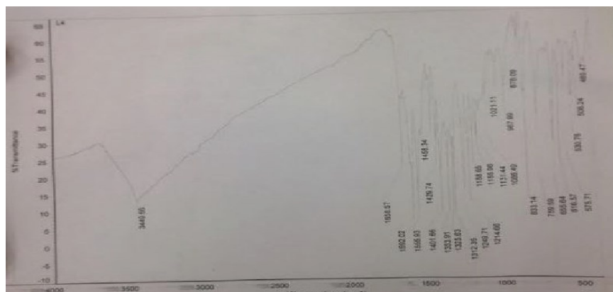
Graph 2. IR spectrum of the Ni(II) complex
