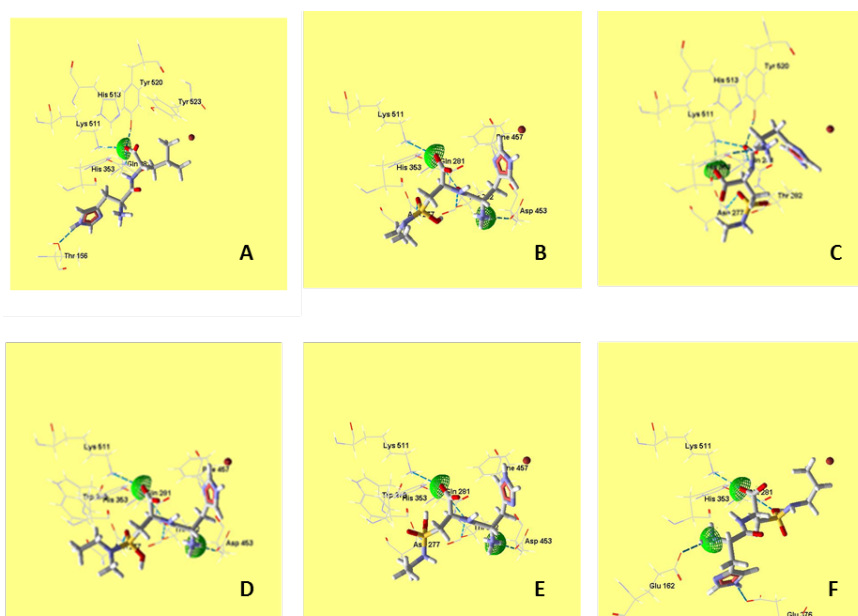
Figure 2. Interactions in the catalytic center of ACE of His-Leu (A), His-sLeu (B), His-sIle (C), His-sNLe 1 (D), His-sNLe 2 (F), and His-sNLe 3 (E).
