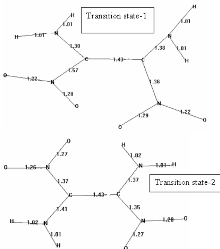
Figure 13. Bond lengths (Å) in transition states-1 and 2 (B3LYP/6-311++G(d,p))
