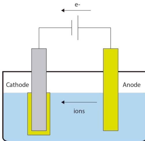
Figure 1. General scheme for electroplating in a liquid bath 4)
