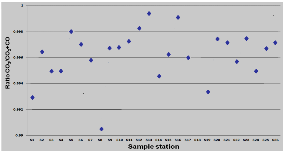
Fig. 4. Ratio of CO 2 /CO 2 +CO in 26 indoor air samples
