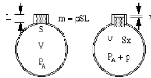
Fig. 4: Air Oscillation
