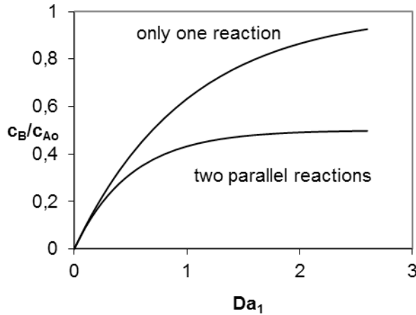
Figure 2. Evolution of the concentration of B with the Damköhler's module of the first reaction
