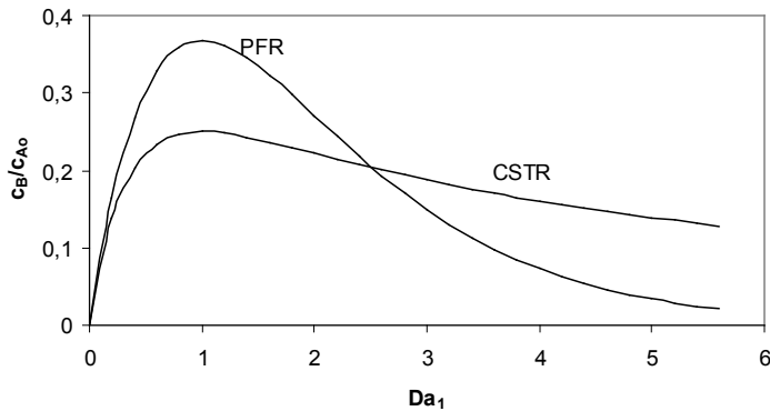
Figure 3. Evolution of the concentration of B with the Damköhler's module first reaction, Da_1 , of the first order series reactions A \xrightarrow{k_1} B \xrightarrow{k_2} C . To facilitate the calculation, it has been considered the case where k_1 = k_2
