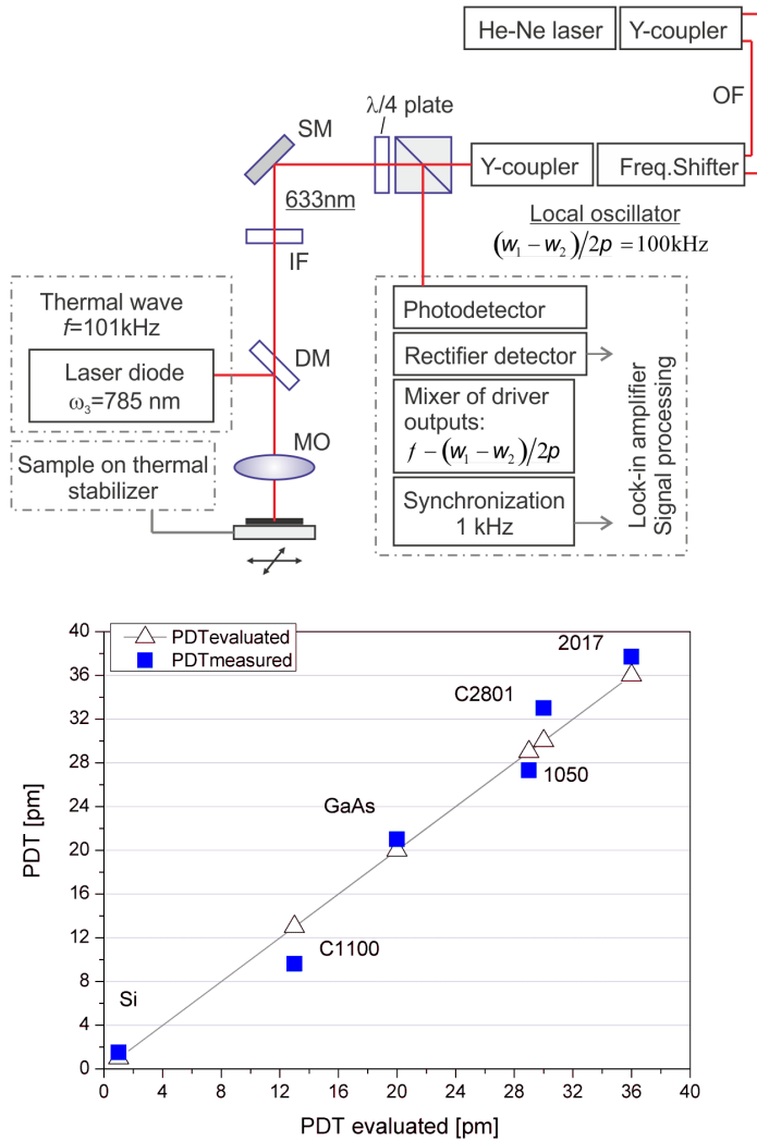
Figure 1. Laser double-heterodyne setup comprising optical fibers (OF), microobjective lens (MO), dichroic mirror (DM), selective mirror (SM) and interference filter (IF) optimized for laser heterodyne wavelength of 632,8 nm; experimental verification for bulk materials: Si, GaAs, Al (1050), Dural (2017), Cu (C1100), CuZn (C2801)
