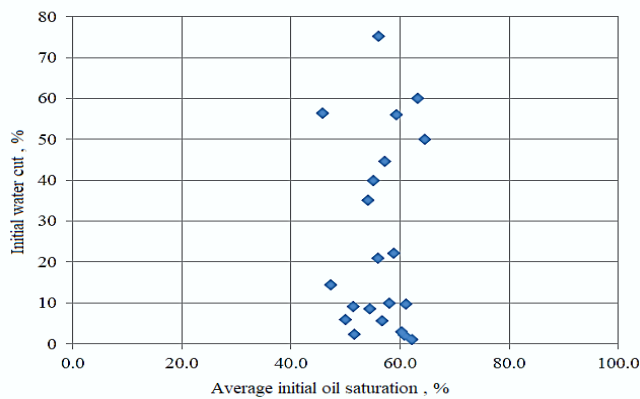
Figure 2. Distribution of initial water cut of wells (first month) and the average initial oil saturation of formations. Vatyogan field, Aptian stage, formation AB1-3 (southwest)
