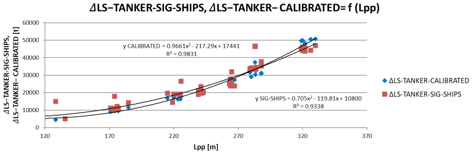
Figure 4. Dependence of the lightship mass for the tankers related to the length of the ship between the perpendiculars
