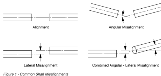
Figure 1. Results of shaft alignment (SDP/SI 2020)
