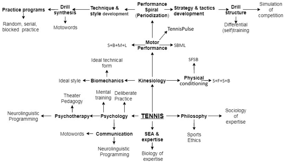
Figure 1. Constituents of expert motor performance, interconnections and the tools provided within the DMCD for their development.
