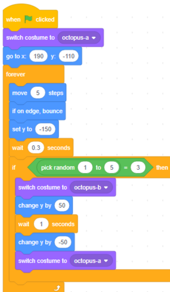
Figure 1. Realization of the sprite Octopus code
